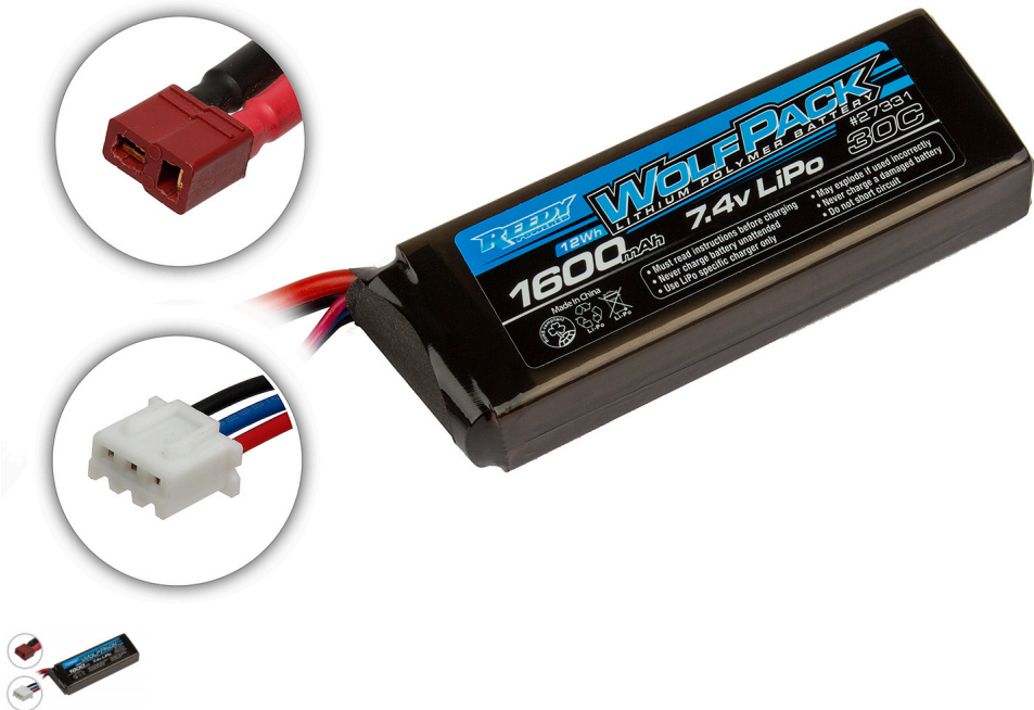
Reedy Wolfpack LiPo 1600mAh 30C 7.4V Battery Pack
